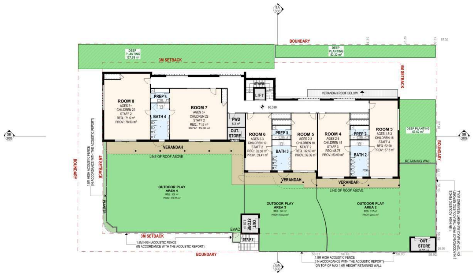
1 FIRST FLOOR 1:200
