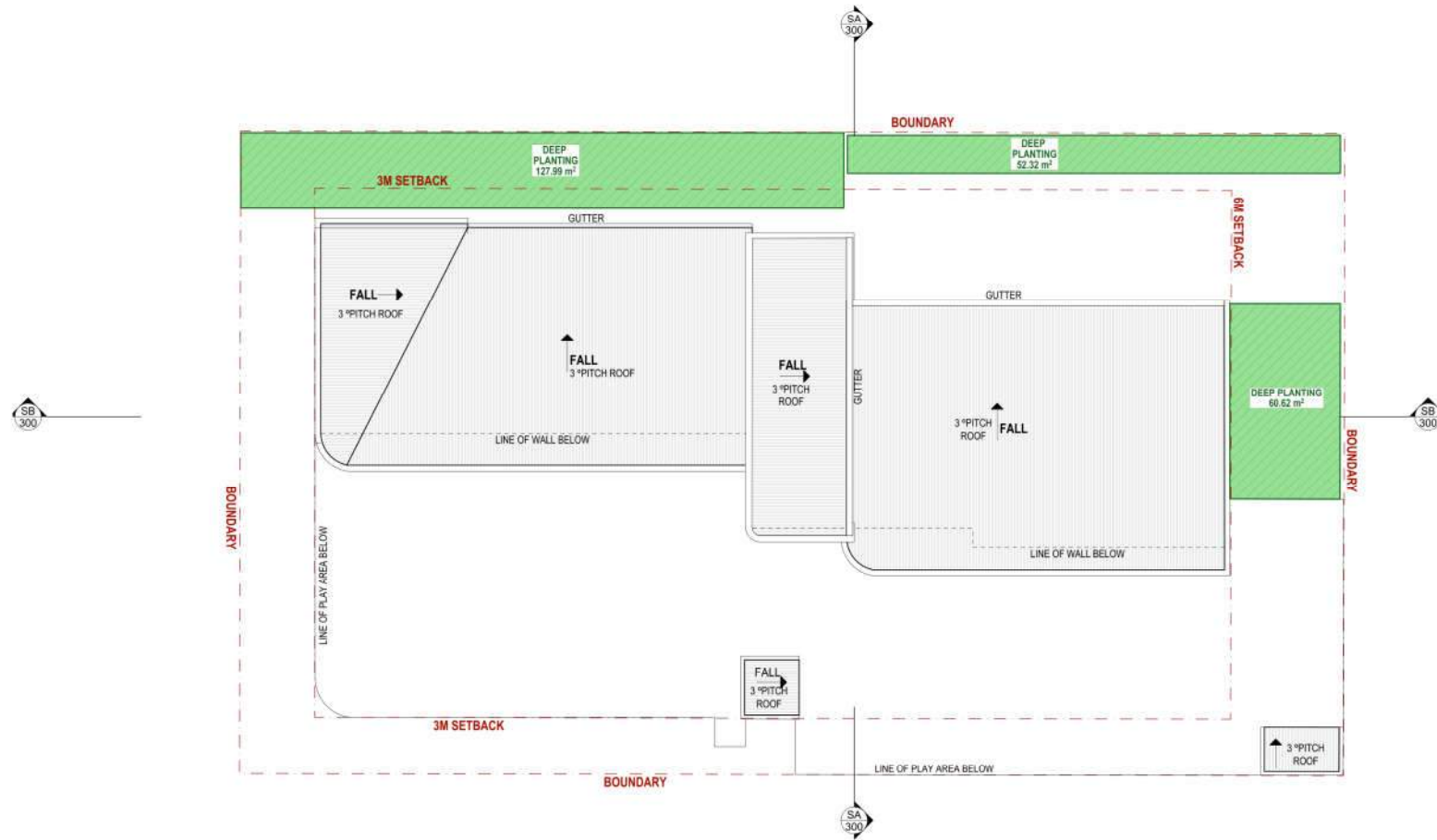
1 ROOF PLAN 1:200
