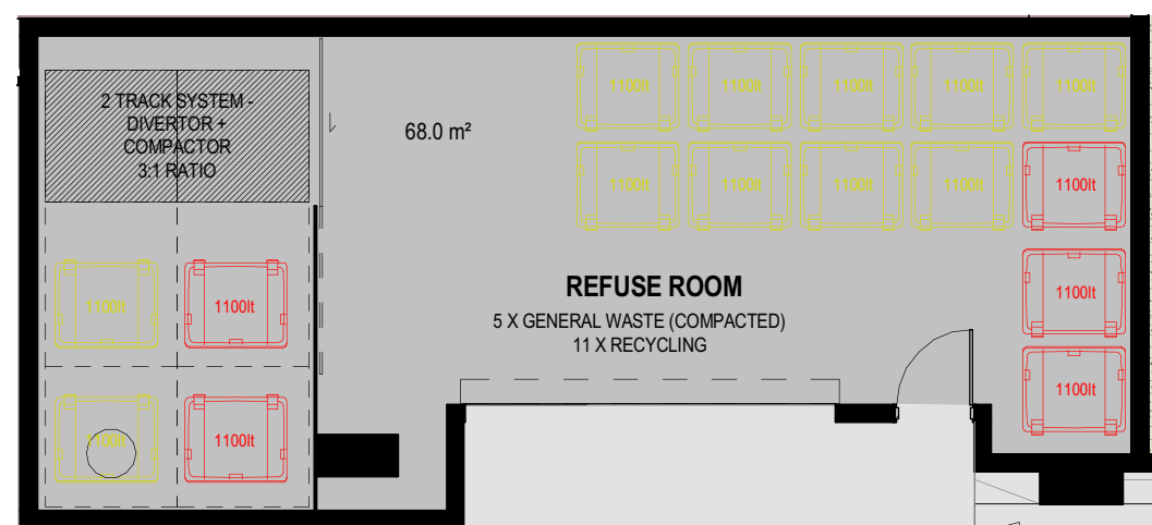
3 BUILDING 2 REFUSE ROOM - DETAIL PLAN 1 : 100
