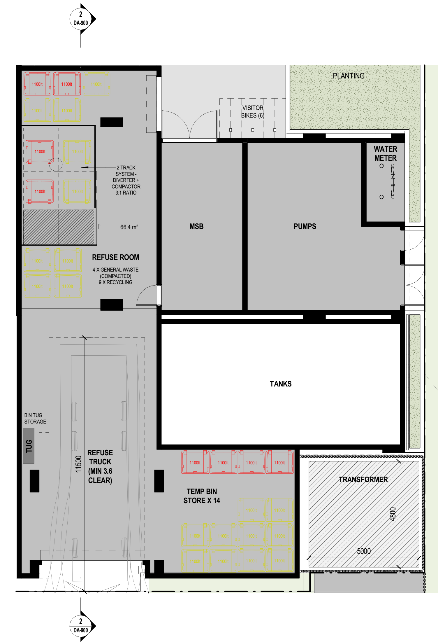
1 BUILDING 1 REFUSE ROOM - DETAIL PLAN 1 : 100
