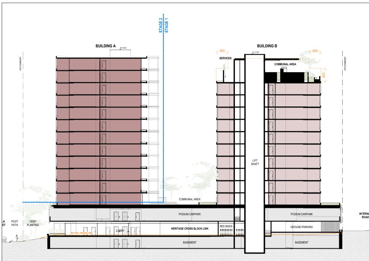
Figure 1 – Development West Elevation
