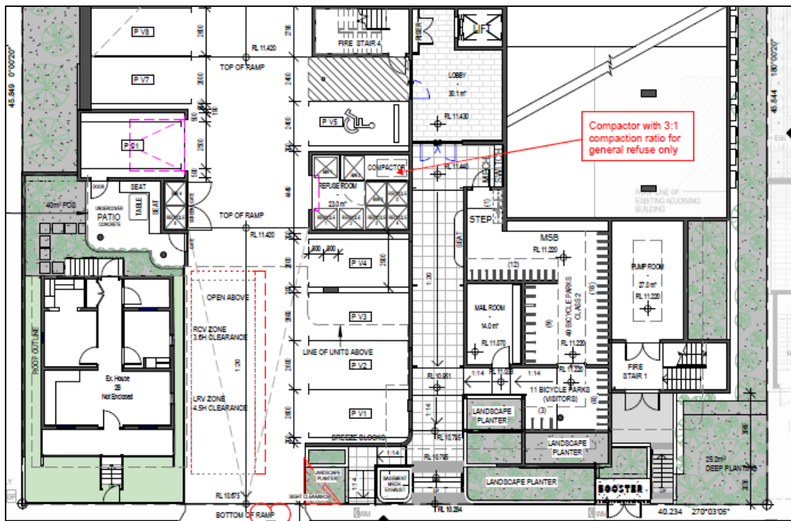
Figure 5 - Approved Ground Floor Plan
