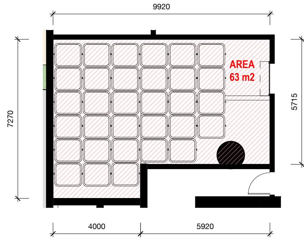
2 Residential Refuse Presentation Room - Ground 1 : 100
