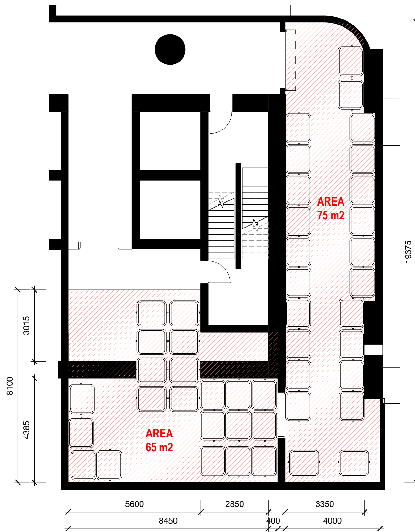
3 Tower C Refuse Room + Precinct Waste Room - Ground 1 : 100
