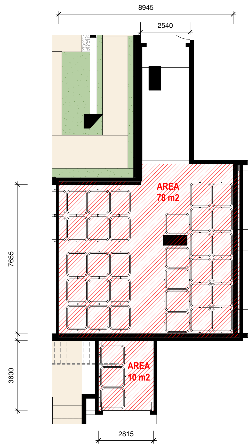
1 Residential Refuse Holding Room - Ground 1 : 100
