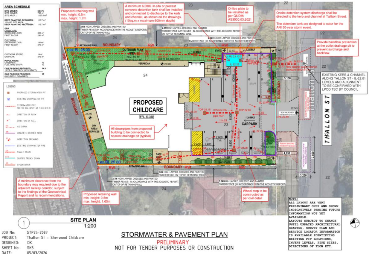
Figure 3.3 - Concept Stormwater Drainage Plan
