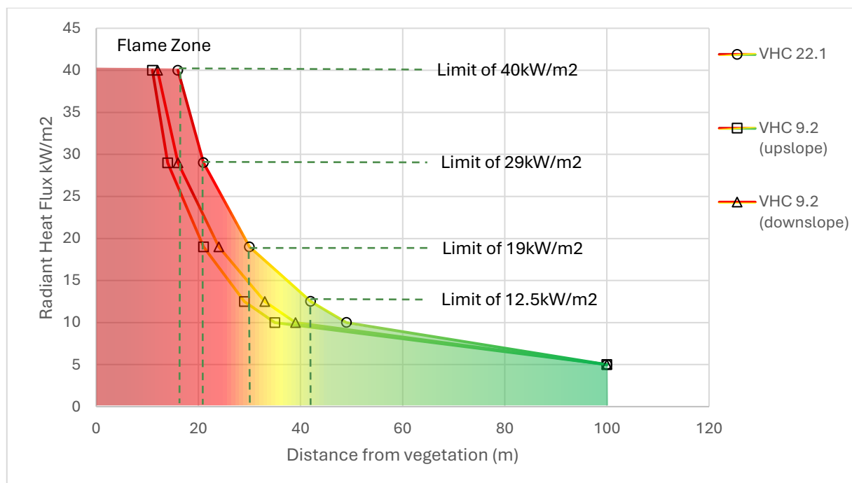
Figure 15 Potential radiant heat flux versus distance from bushland areas
